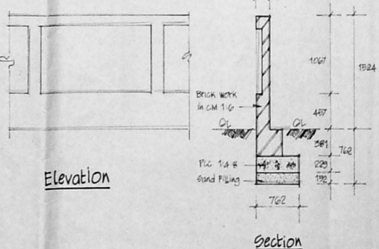
COMPOUND WALL DETAIL
