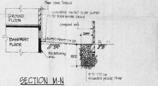
SECTION M-N
