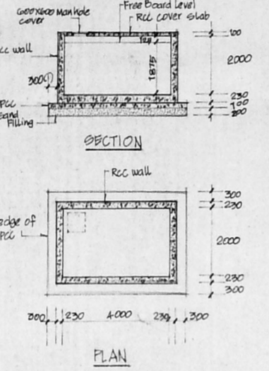
SUMP DETAIL
