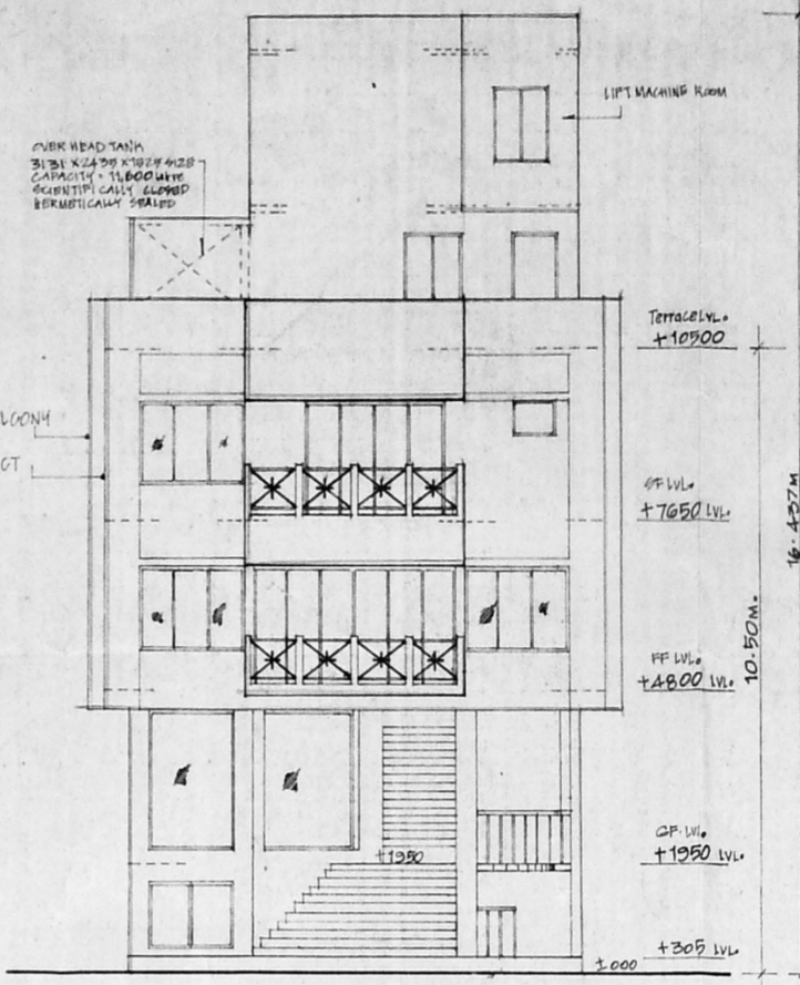
FRONT ELEVATION
